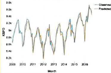
US Gasoline Demand observed vs. predicted
